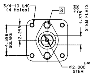
ACTUATOR MOUNTING: 8"
