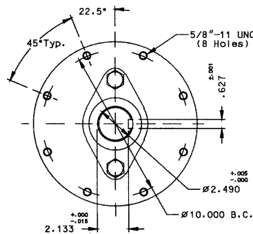
ACTUATOR MOUNTING: 10" & 12"
