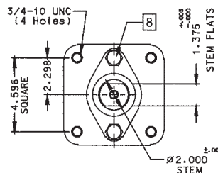
ACTUATOR MOUNTING: 8"
